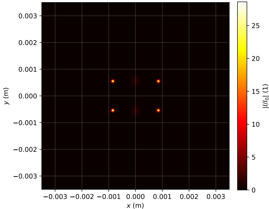
Intensity profile I(x, y, z = 0.716)/I_0 , P_{in}=7.0P_{cr} , artificial time
